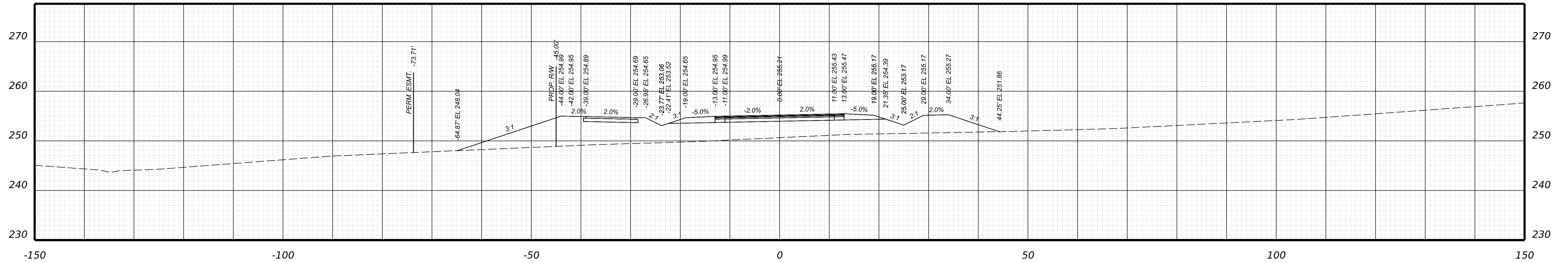
Bailey Bridge Connector STA 112+75.00
