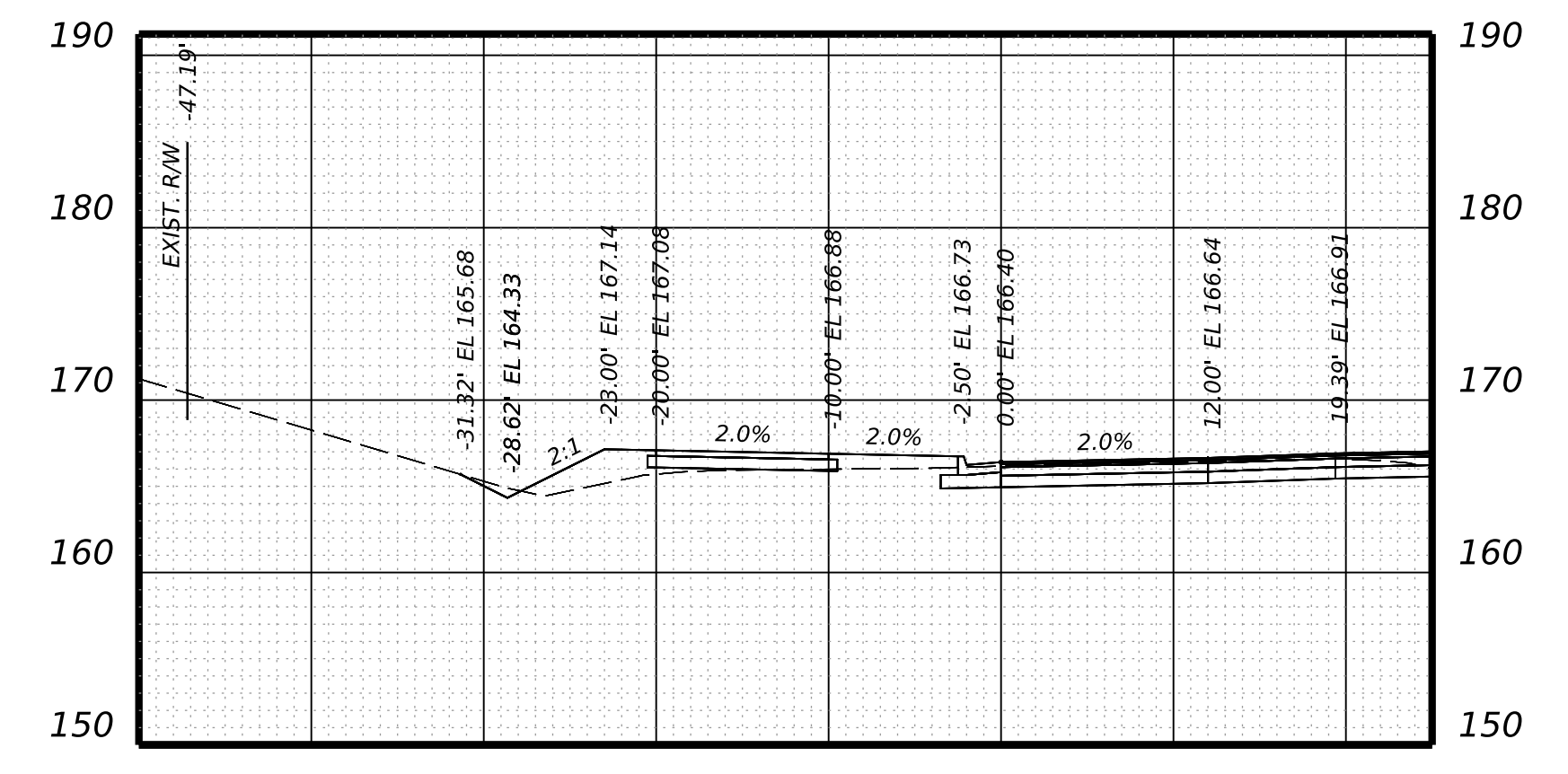
Brad McNeer Parkway Bypass STA 34+00.00
