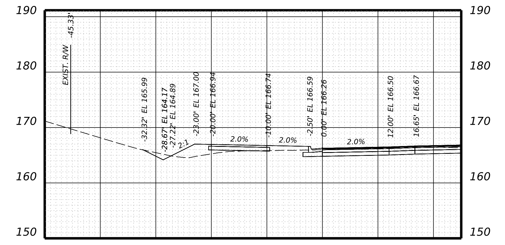
Brad McNeer Parkway Bypass STA 34+25.00
