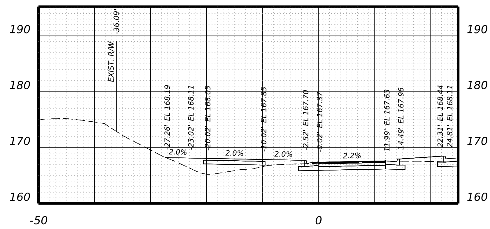
Brad McNeer Parkway Bypass STA 32+25.00
