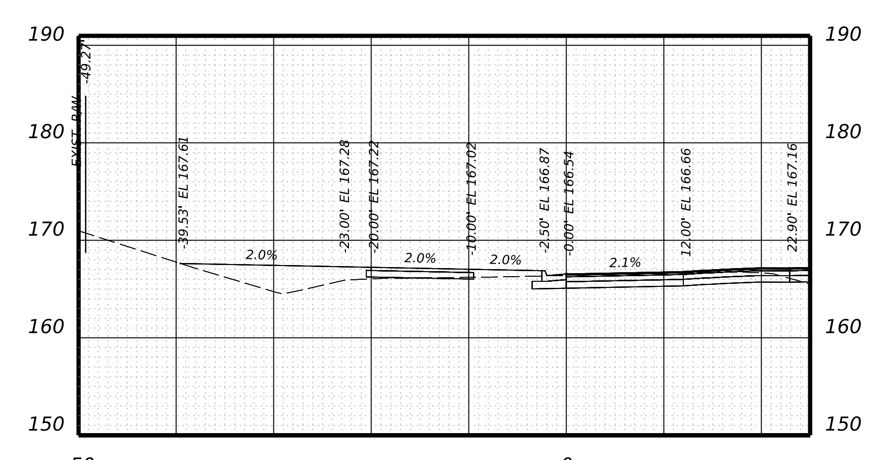
Brad McNeer Parkway Bypass STA 33+75.00
