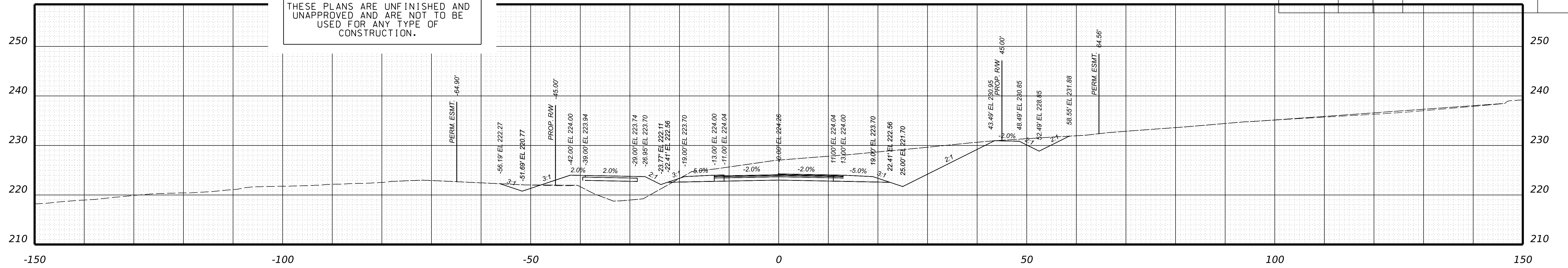
Bailey Bridge Connector STA 139+50.00
